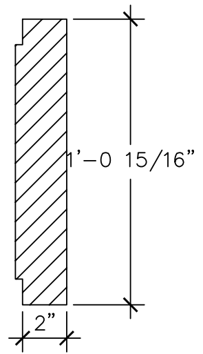
CROSS-SECTION A-A
