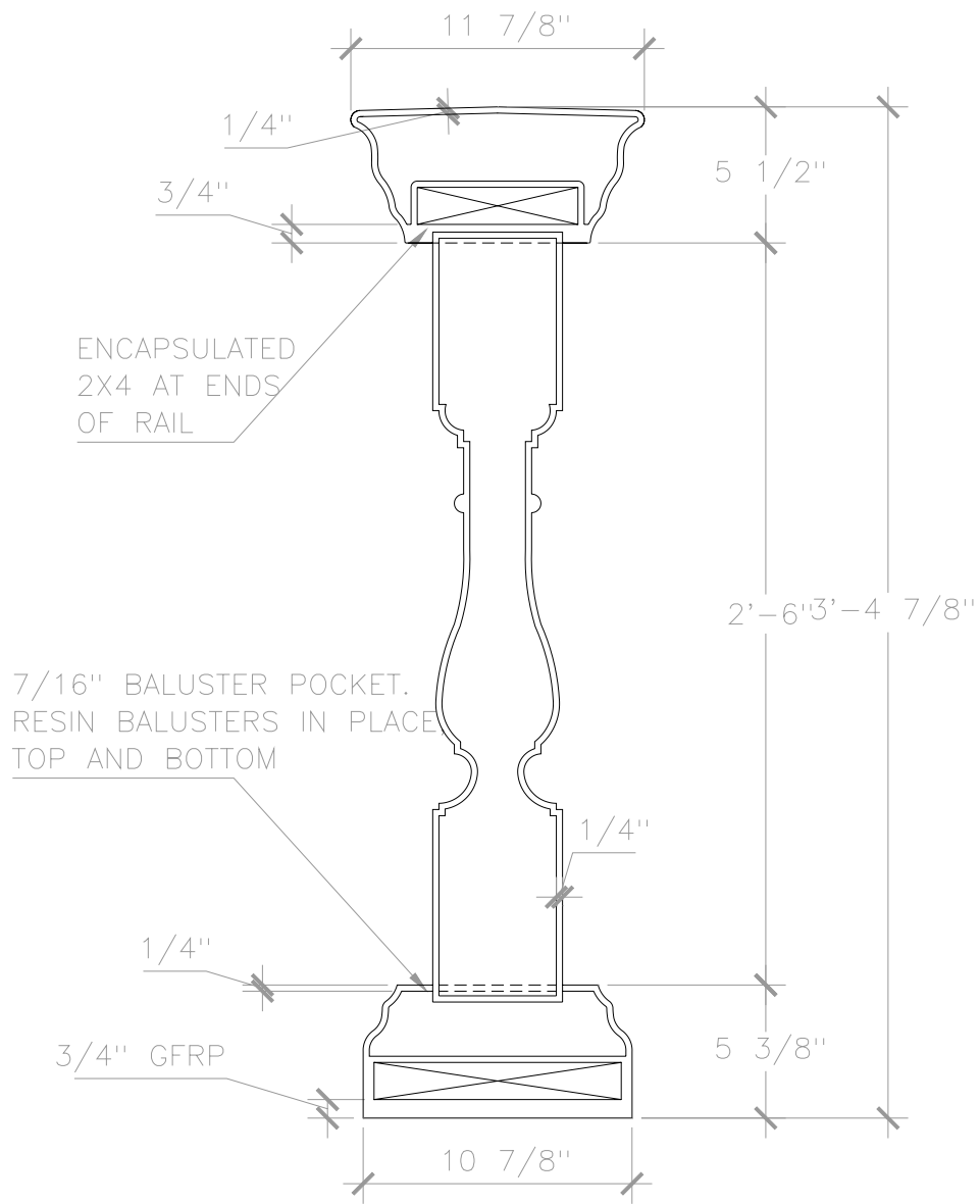
END VIEW
