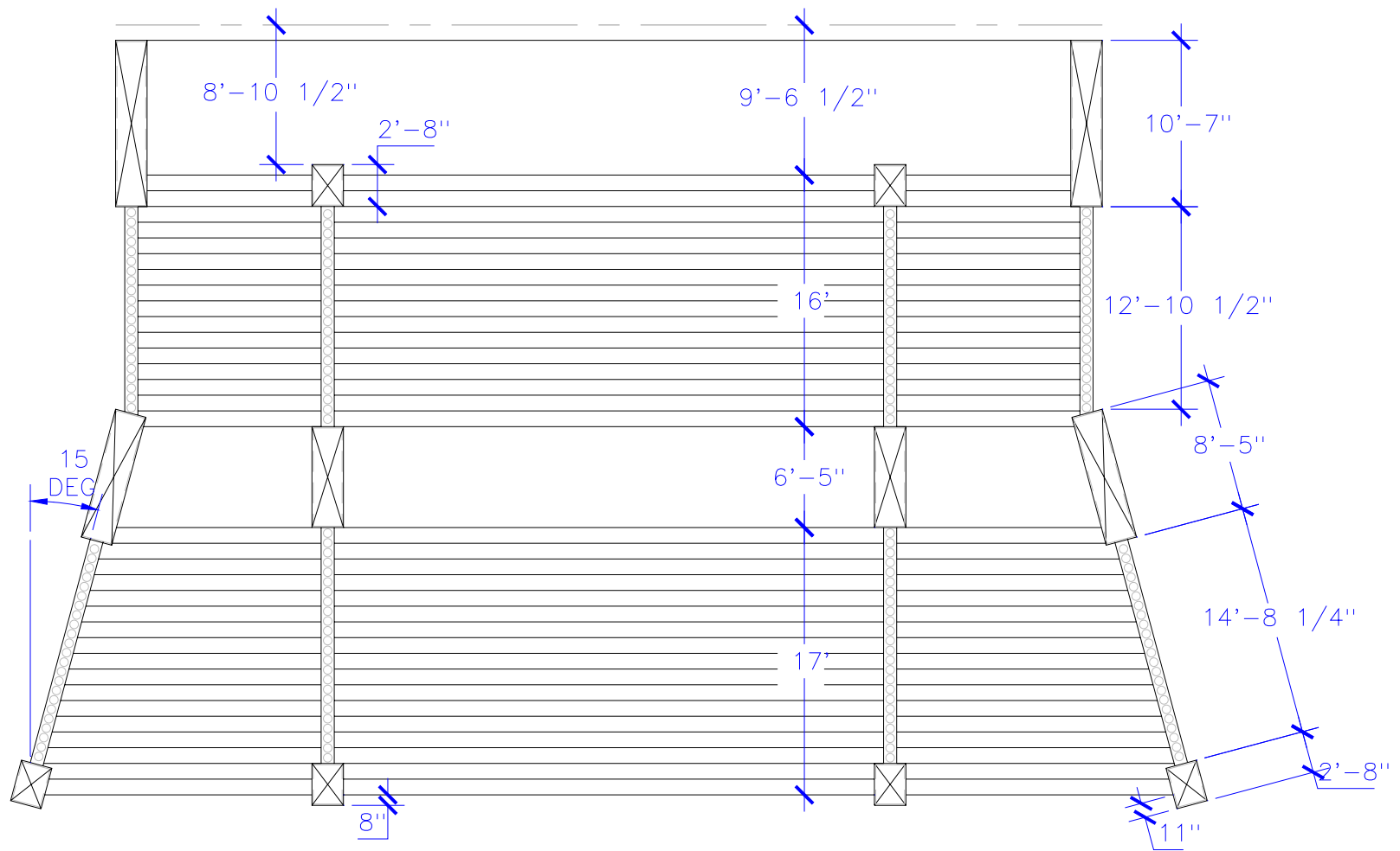
PLAN VIEW
