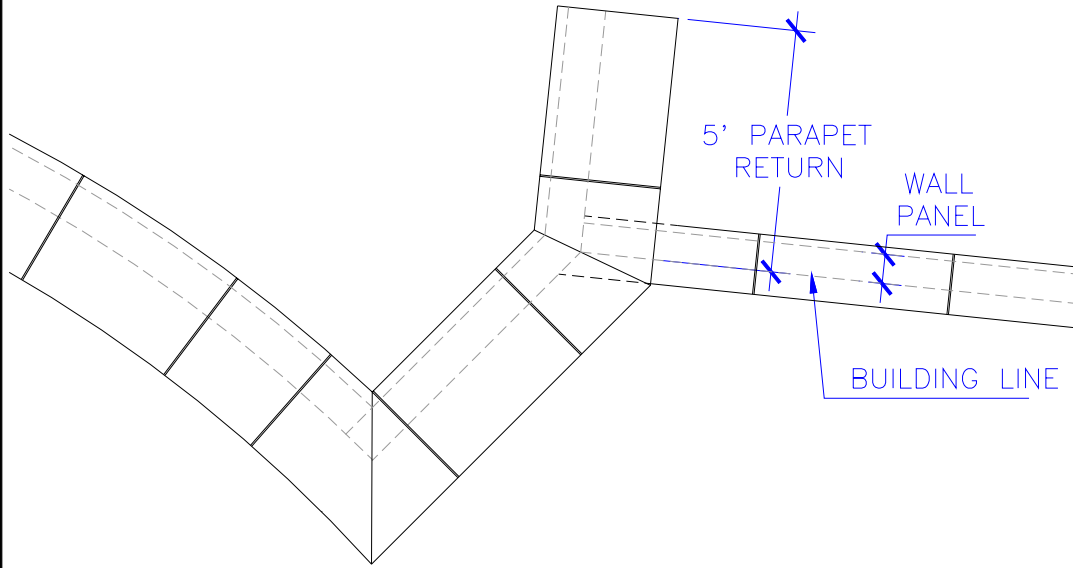
DETAIL - A - TOP VIEW
