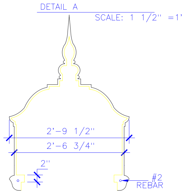
SECTION A
