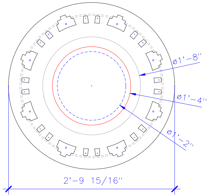
SECTION A
