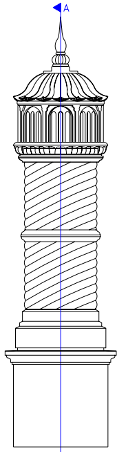
SECTION A ELEVATION / SECTION SCALE: 1/4" = 1'
