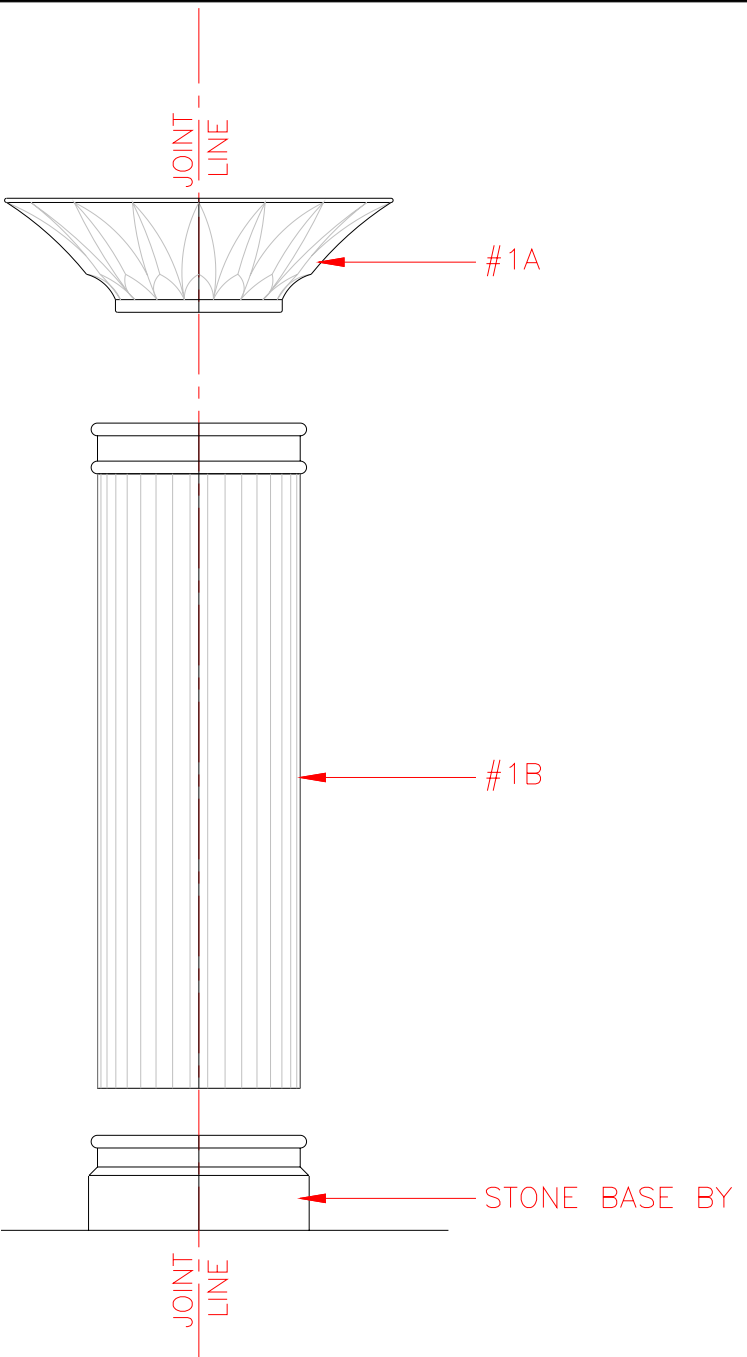
B SIDE 1/4" = 1'-0"
