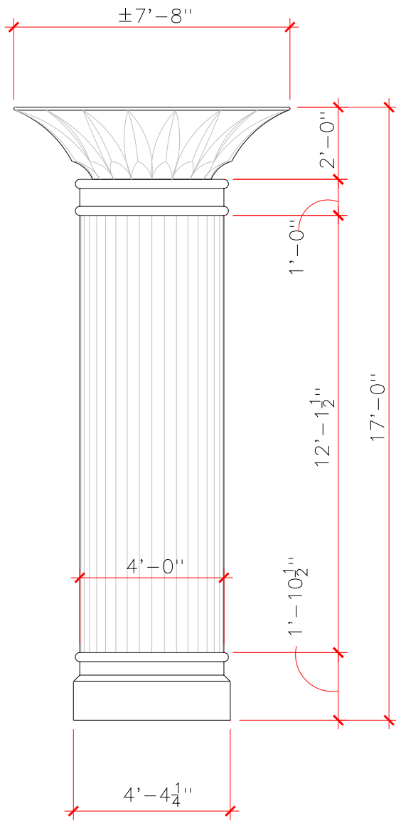
A FRONT 1/4" = 1'-0"
