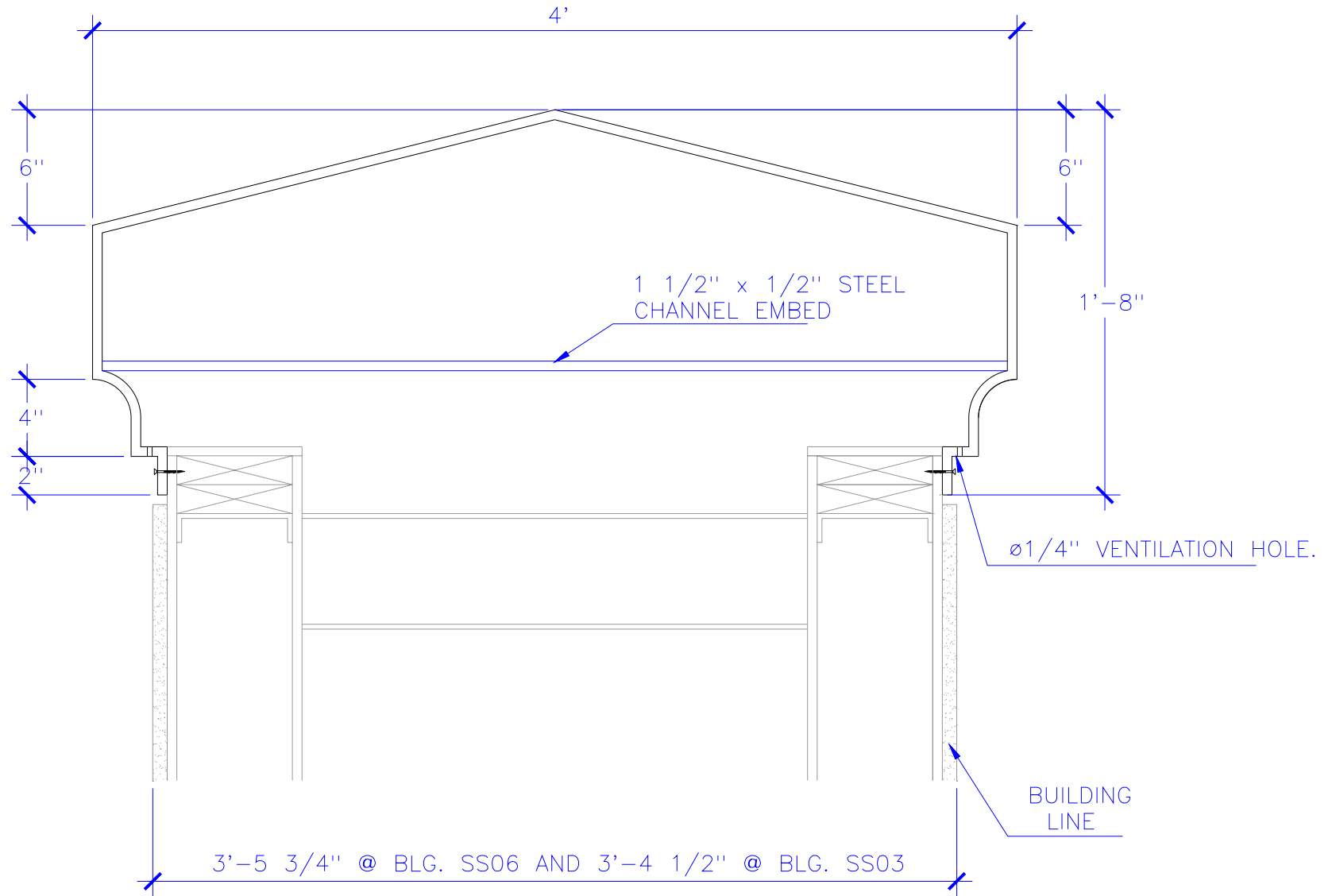
- D - CORNICE TYPICAL SECTION
