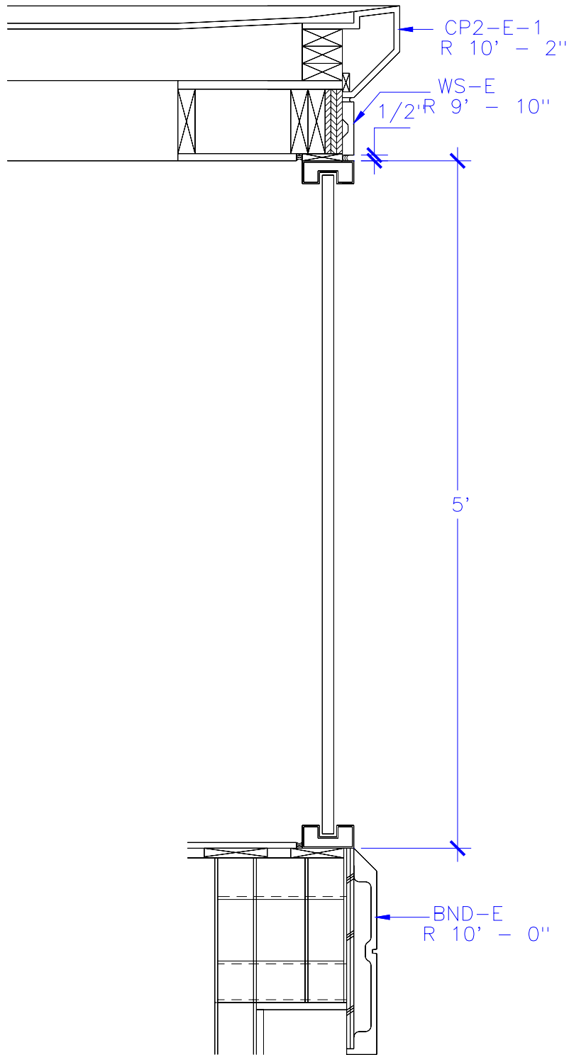
SECTION E AT WINDOW, SIMILAR
