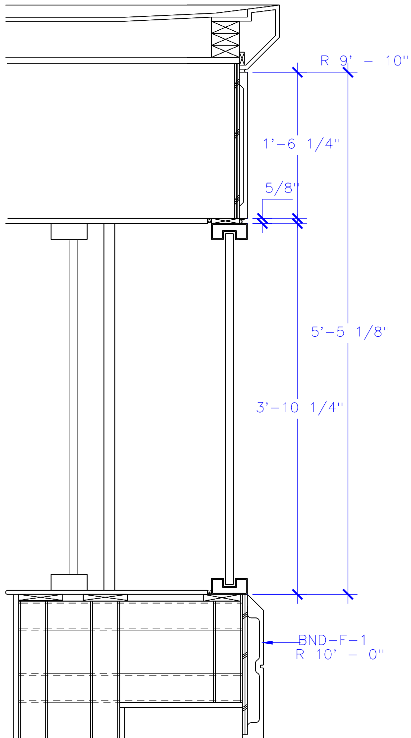
SECTION A AT WINDOW
