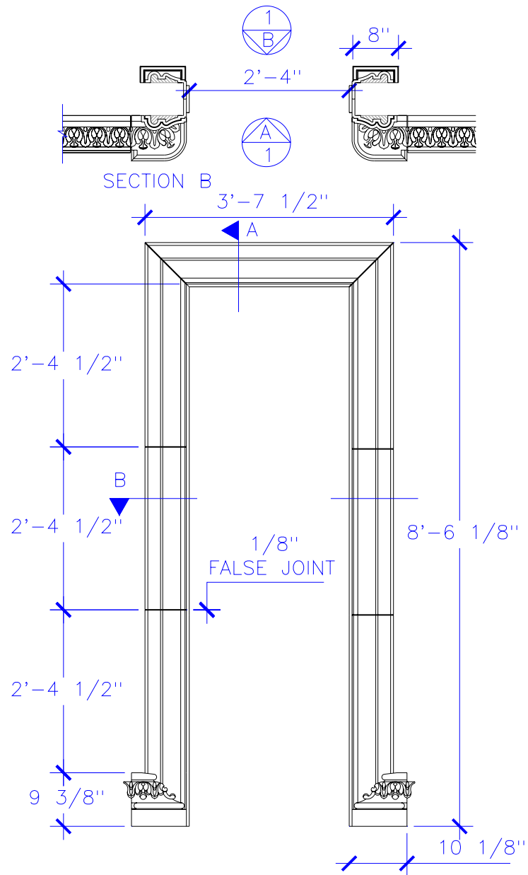
VIEW A
