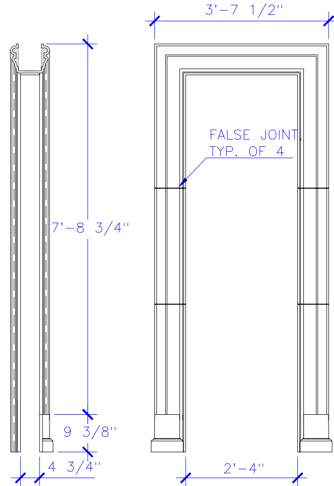
SECTION A
