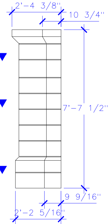
PART LAYOUT SCALE: 3/16" = 1'
