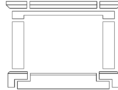
PART LAYOUT SCALE: 3/16" = 1'
