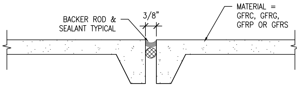
FLANGE JOINT DETAL A
