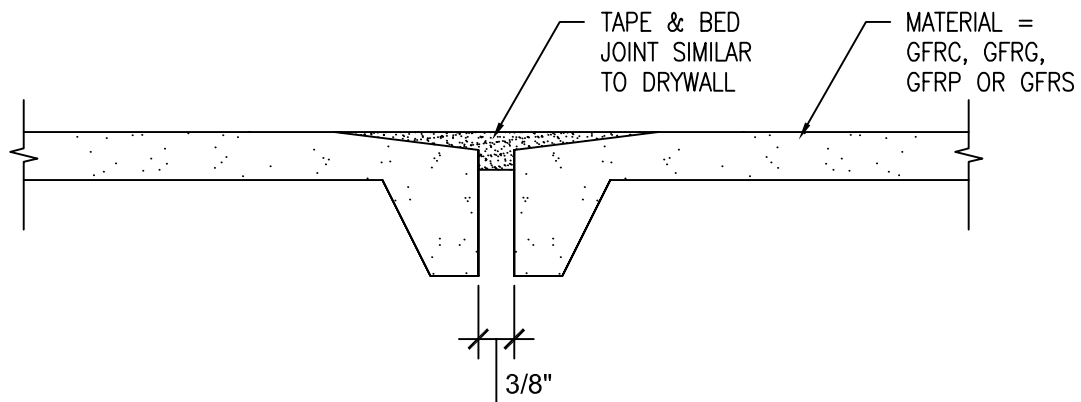
TYPICAL FLANGE JOINT DETAIL SCALE: 6" = 1'-0"
