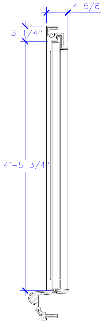
SECTION B
