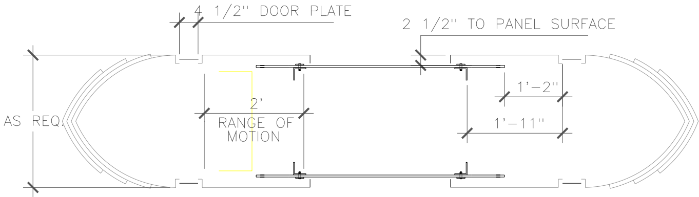
UPPER ASSEMBLYS
