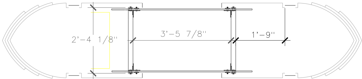
LOWER ASSEMBLYS
