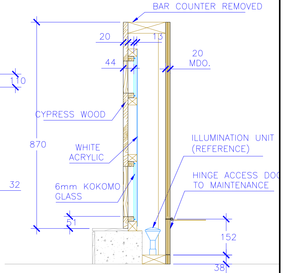
BAR PANEL SECTION - E - SCALE : 1 = 10
