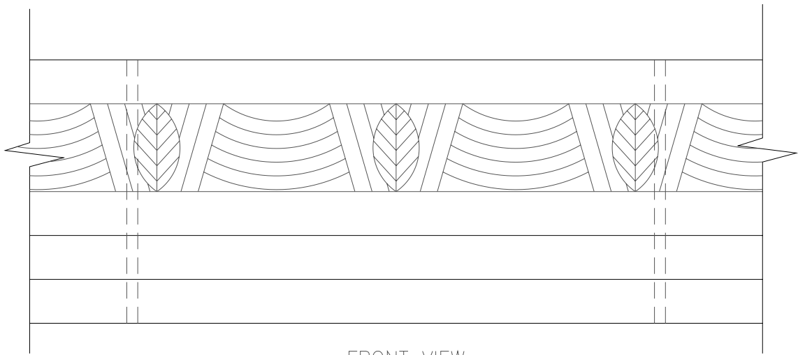
FRONT VIEW
