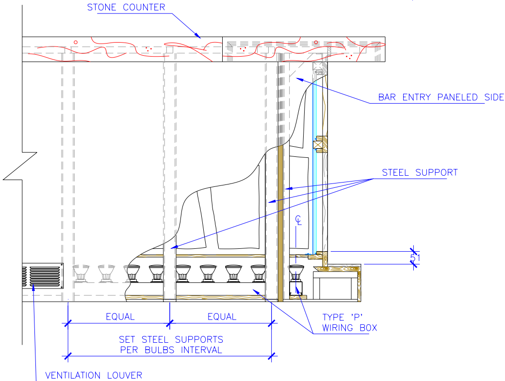
BAR ASSEMBLY, DETAIL - H - SCALE : 1 = 10
