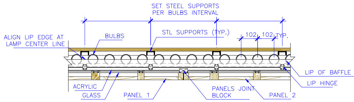
BAR ASSEMBLY, DETAIL - F - SCALE : 1 = 10
