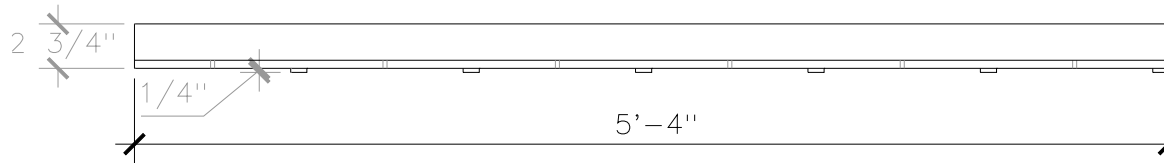
DETAIL A
