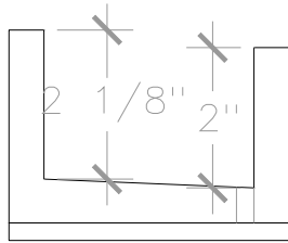
DETAIL A 4" = 1'
