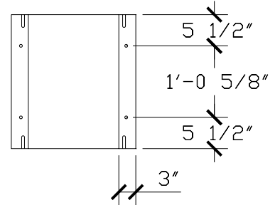
FASTENER DETAIL
