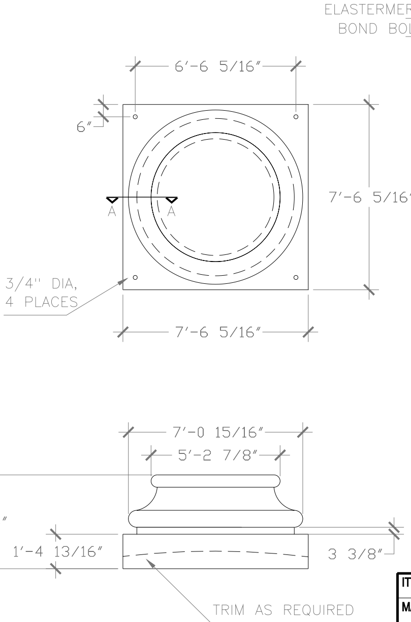
MOUNTING DETAILS
