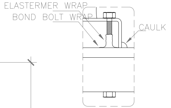
MOUNTING DETAILS
