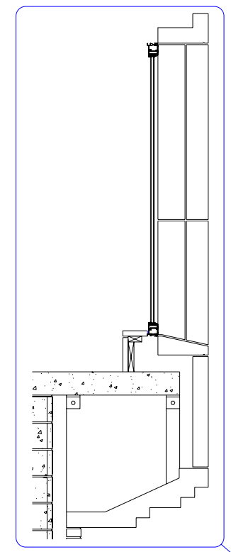
SECTION A SCALE 1/2" = 1'
