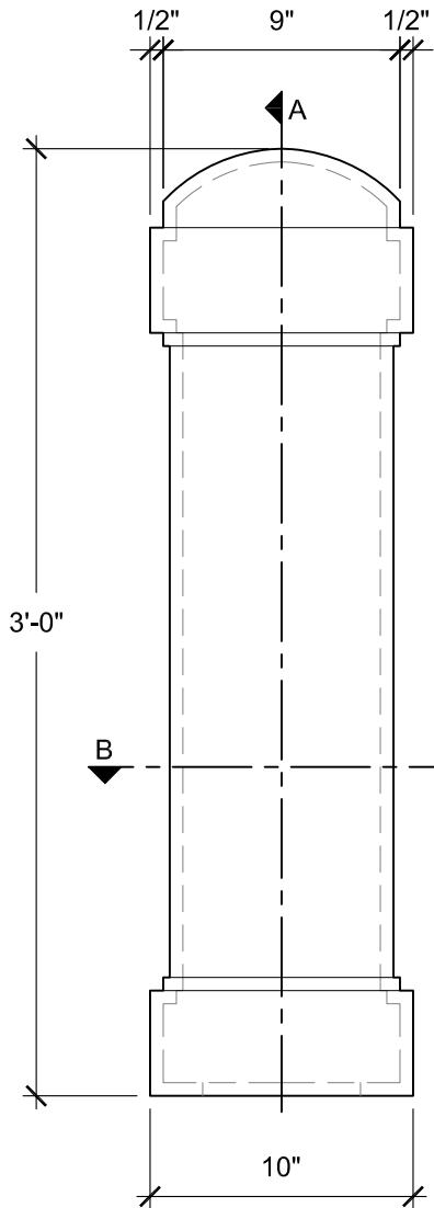
FRONT VIEW SCALE: 1 1/2" = 1'-0"
