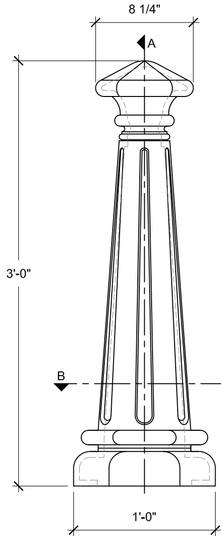
FRONT VIEW SCALE: 1 1/2" = 1'-0"
