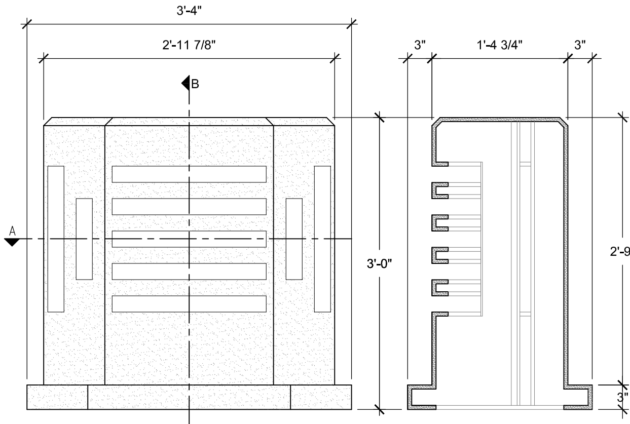
FRONT VIEW SCALE: 1"= 1'-0"
