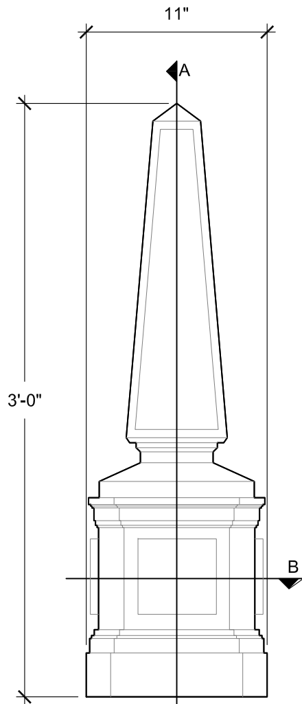
FRONT VIEW SCALE: 1 1/2"= 1'-0"
