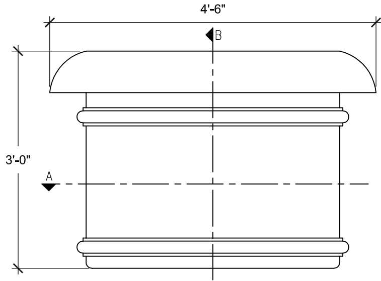
FRONT VIEW SCALE: 3/4" = 1'-0"
