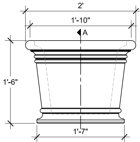
FRONT VIEW SCALE: 1"= 1'-0"
