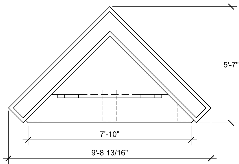
SECTION A
