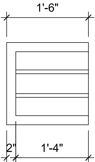
SIDE ELEVATION
