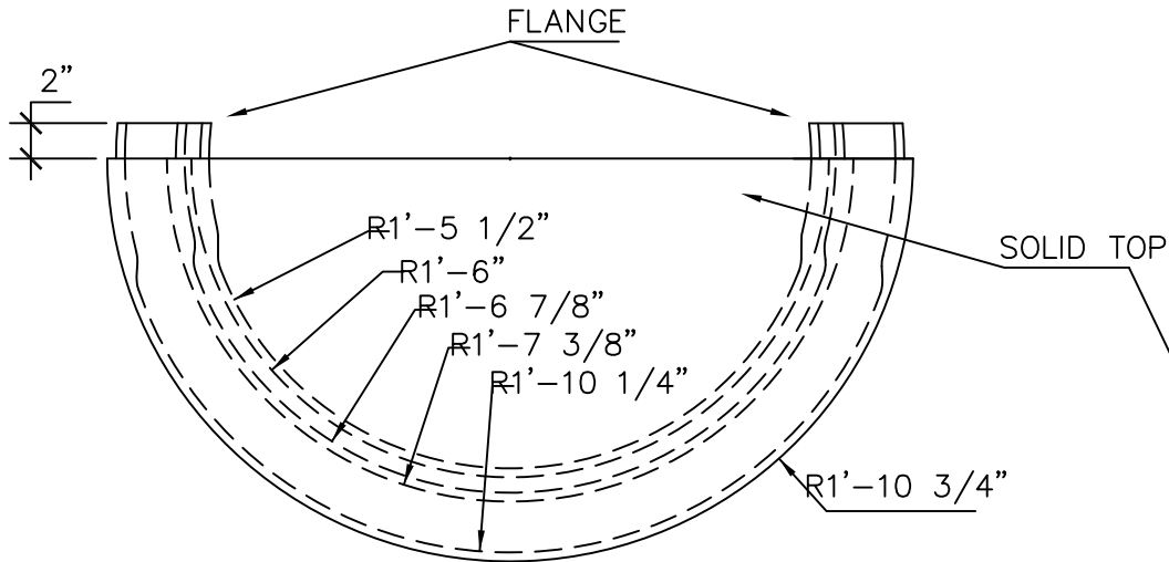
TOP VIEW
