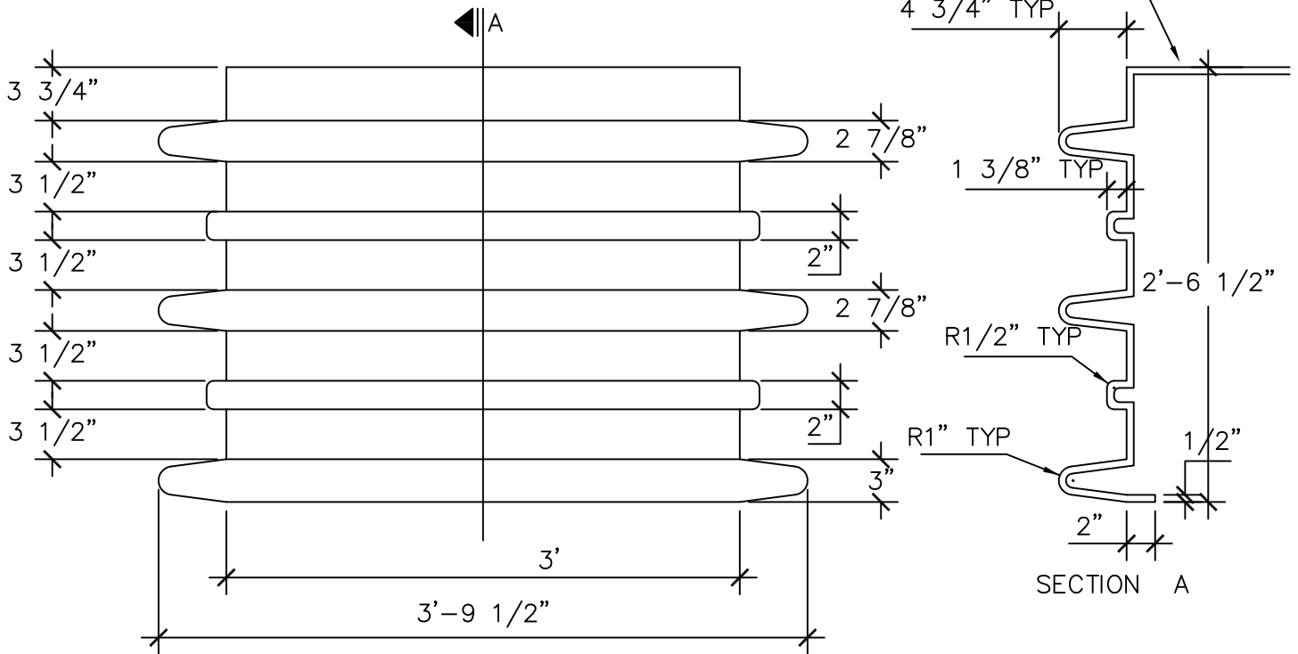
FRONT VIEW
