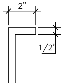
SECTION A SCALE 3" = 1'
