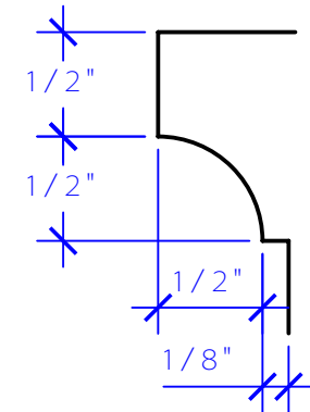
SECTION B SCALE: FULL SIZE
