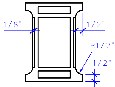
SECTION A
