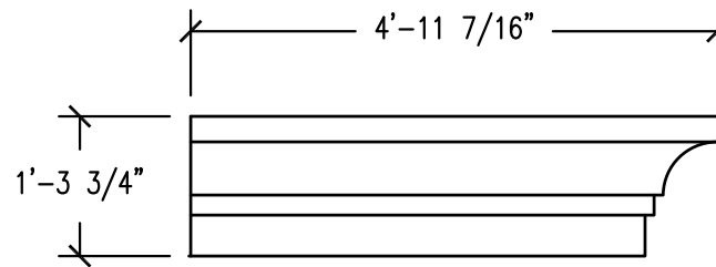
09 CORNICE SECTION
