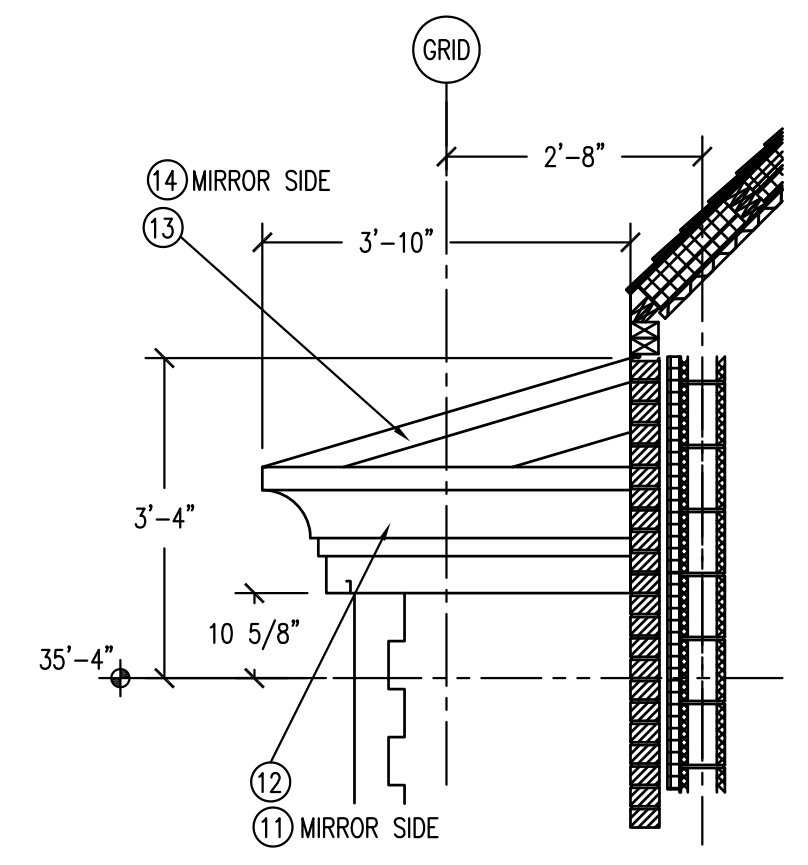
2 ELEVATION DETAIL SP1 1/2" = 1'
