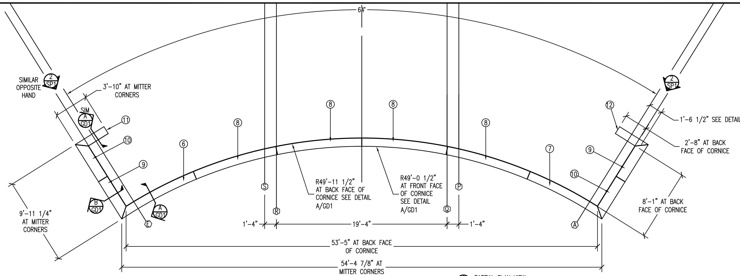
1 PARTIAL PLAN VIEW SP1 3/16" = 1'
