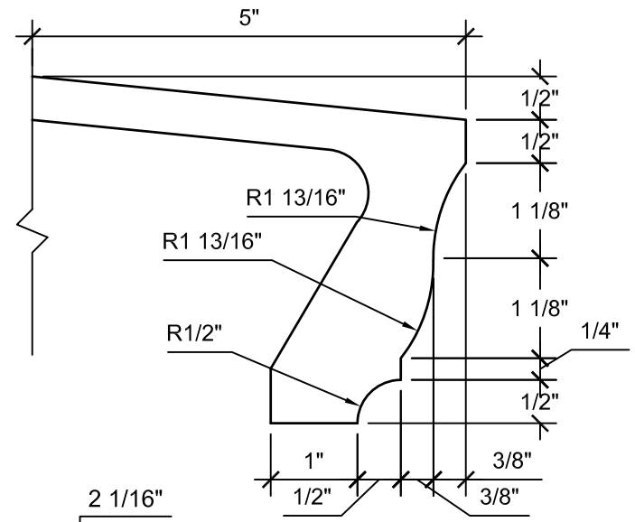
ENLARGED PROFILE
