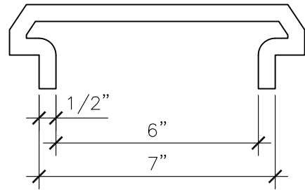
SECTION A
