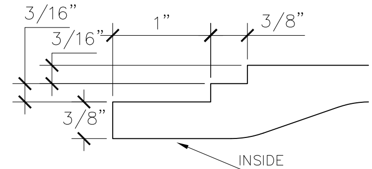
SECTION A, SPACER FLANGE FULL SIZE
