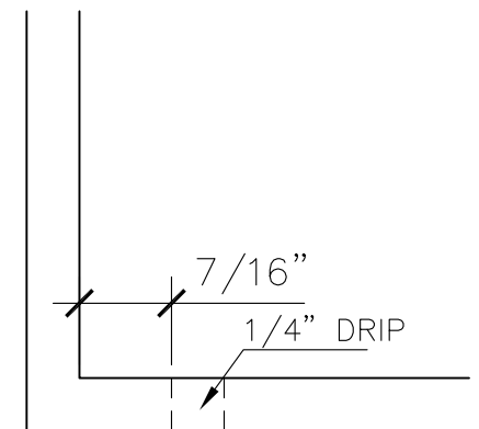
DETAIL A SCALE: FULL SCALE
