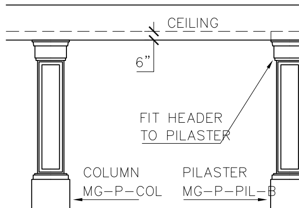
SOUTH ELEVATION AT MANAGERS OFFICE.
