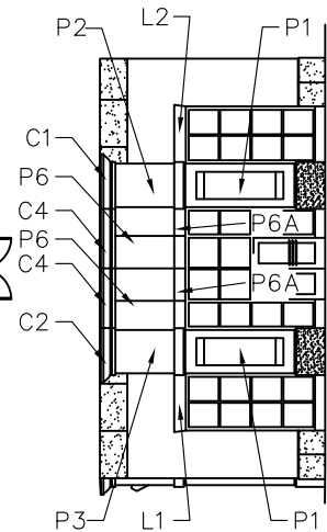
EAST ELEVATION
