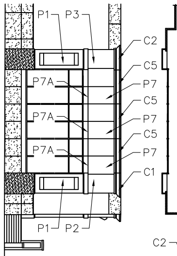
WEST ELEVATION
