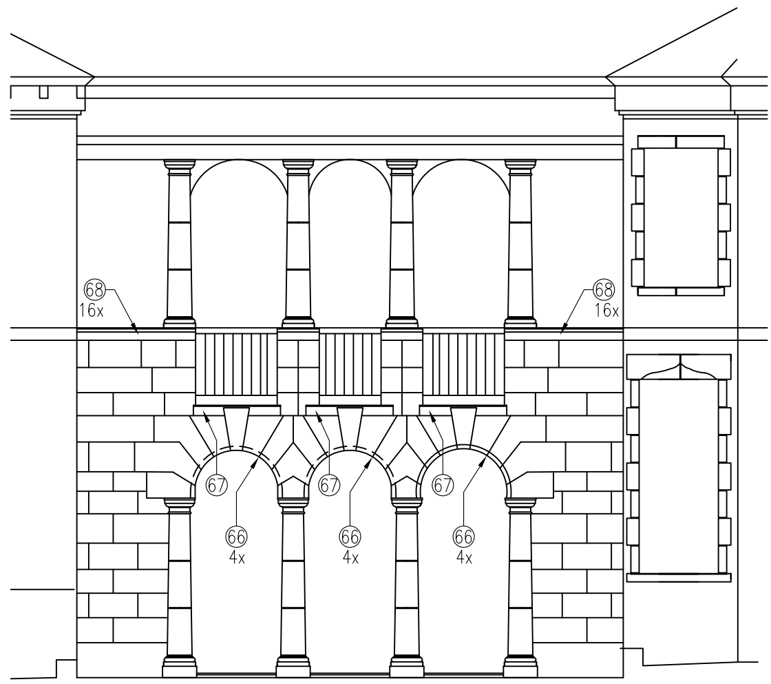
FIRST FLOOR SECTION VIEW 3/16" = 1'
