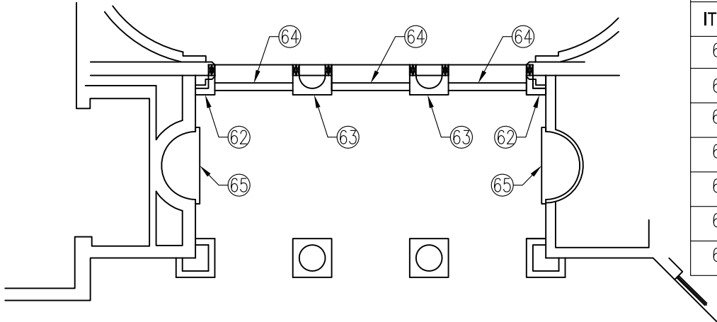
FIRST FLOOR SECTION VIEW 3/16" = 1'
