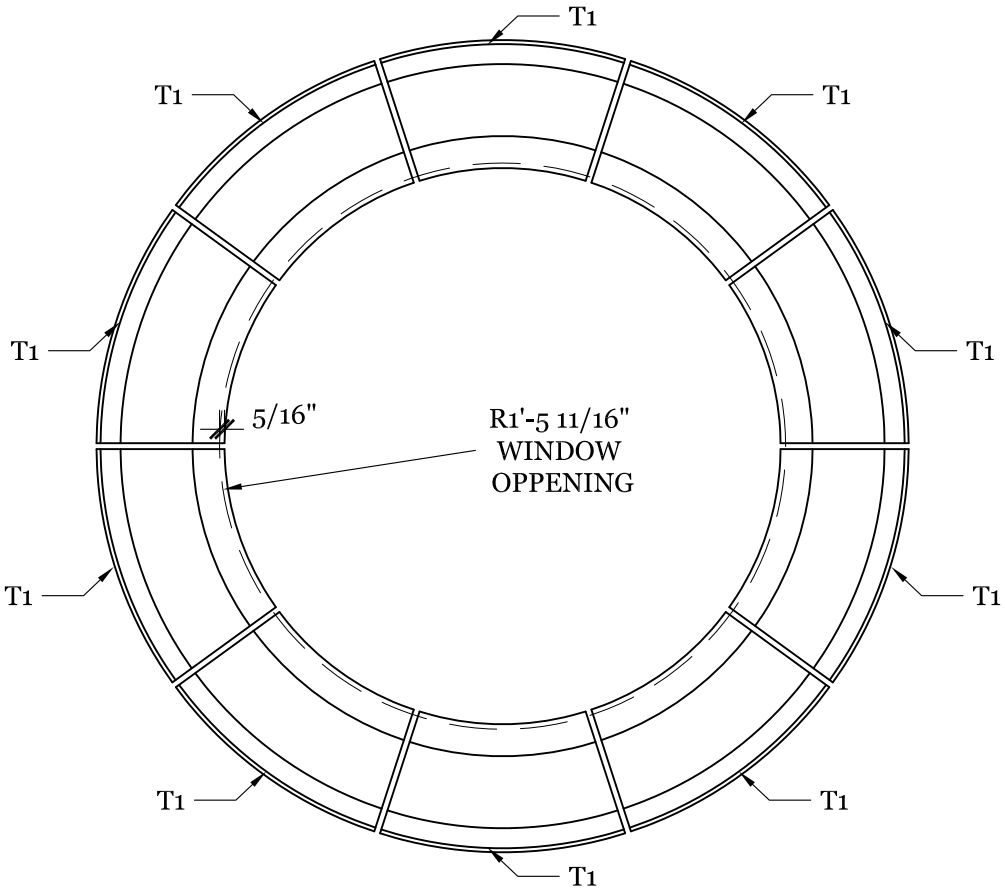
WINDOW 217 TRIM 1" = 1'
