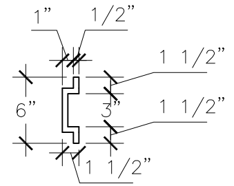
SECTION A
