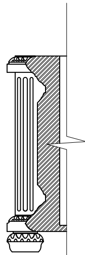
SECTION A
