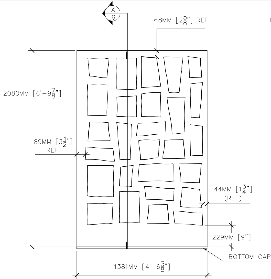
WALL PANEL "B2" SCALE: 1 = 20
