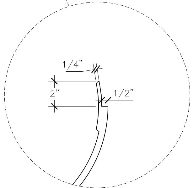
FLANGE DETAIL
