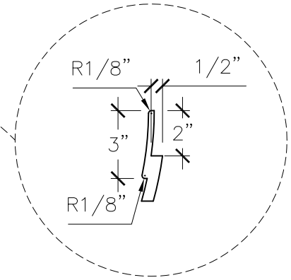
ENLARGED FLANGE DETAIL
