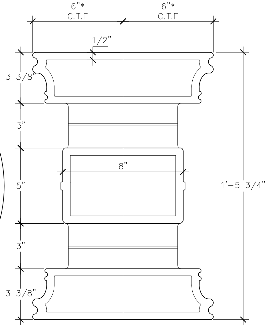
SECTION A
